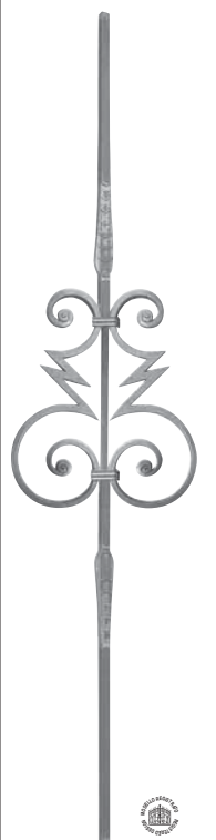
Art. GDI95/7 ∅ 14 x 14 mm H 1000 mm L 215 mm
